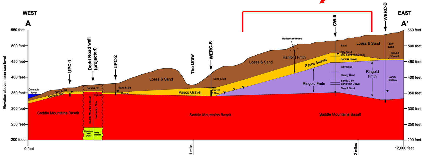
Subsurface Profile A-A'
